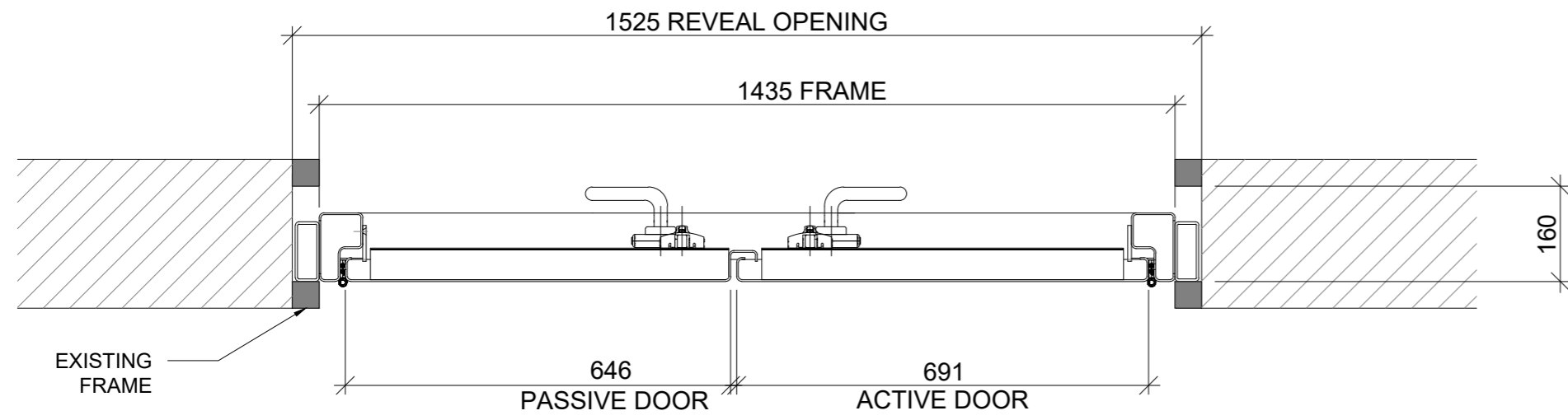
PLAN VIEW
